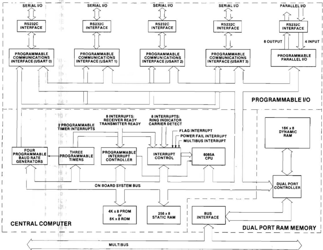
Figure 1. iSBC 544 INTELLIGENT COMMUNICATIONS CONTROLLER BLOCK DIAGRAM
