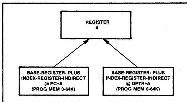
Figure 2.17 Program Memory Move Operations
