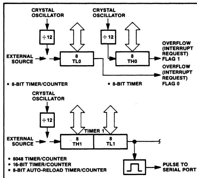
Figure 2.4.B. Timer/Event Counter Mode 3
