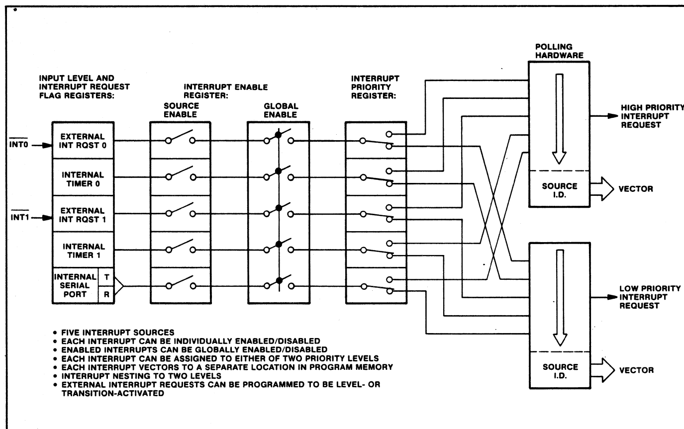
Figure 2.2. 8051 Interrupt System
