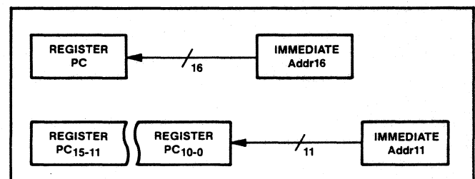
Figure 2.28. Unconditional Branch Operations
