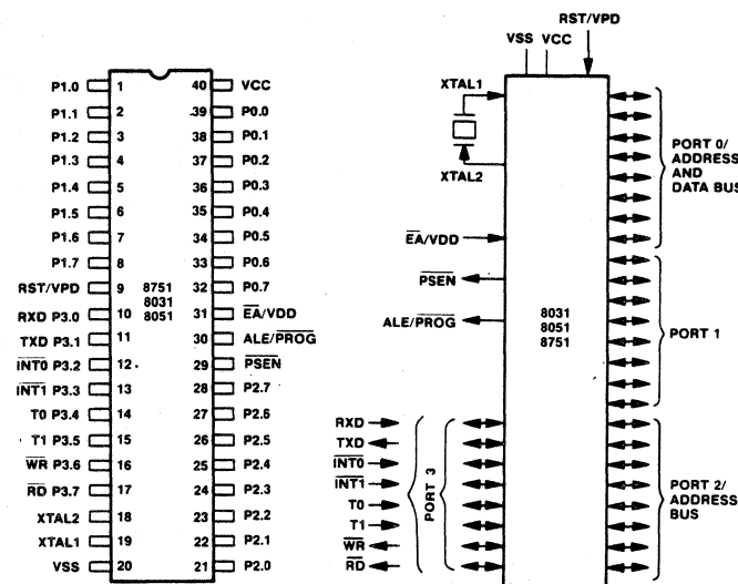
Figure 1. Pin Configuration
