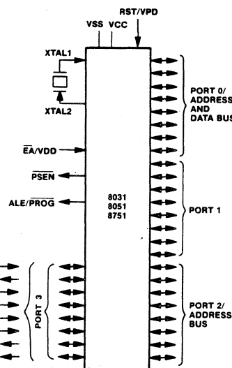
Figure 2. Logic Symbol
