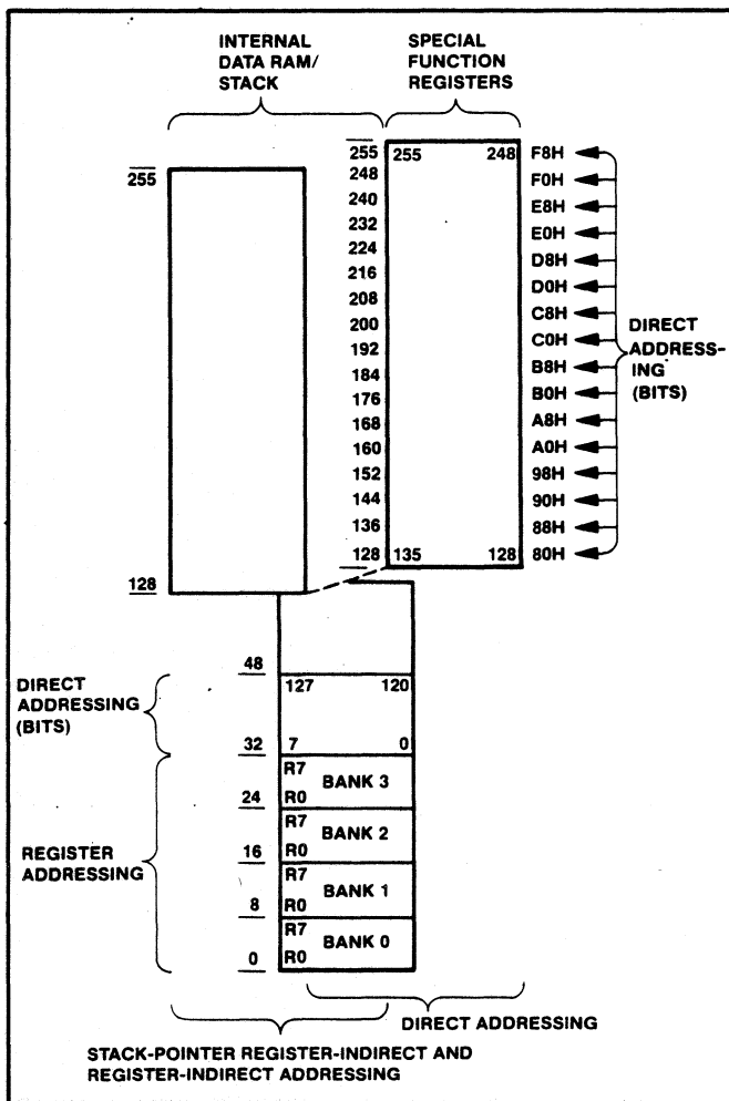
Figure 2.16. Addressing Operands in Internal Data Memory
