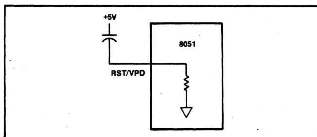
Figure 2.54. Power-On Reset
