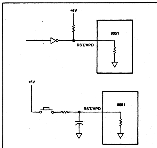
Figure 2.55. External Reset
