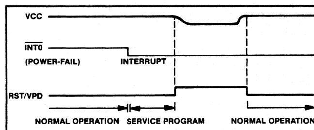
Figure 2.56. Power-Down Sequence
