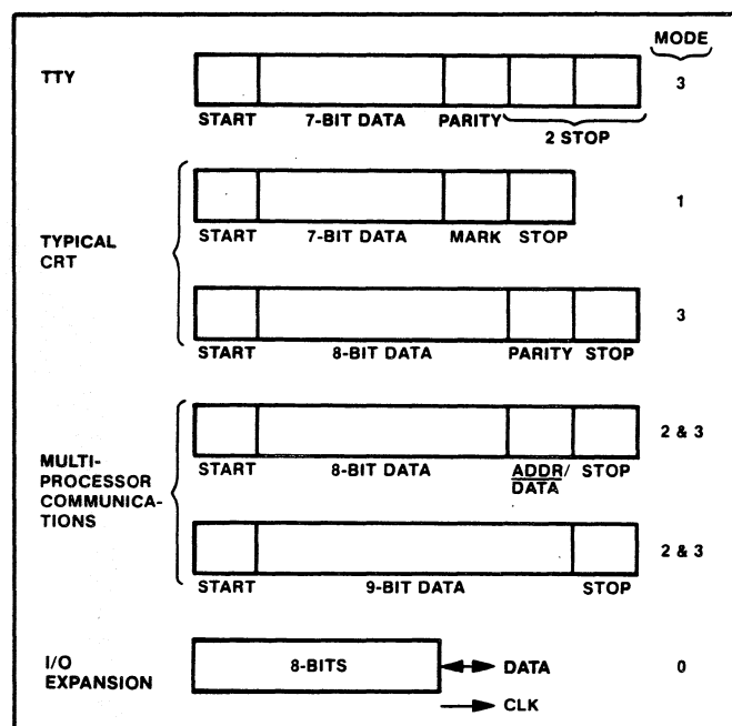
Figure 2.9. Typical Frame Formats
