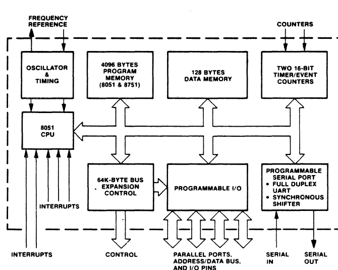
Figure 3. Block Diagram
