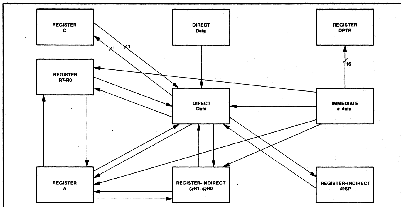
Figure 2.19. Internal Data Memory Move Operations
