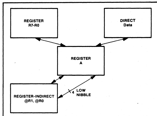
Figure 2.20. Internal Data Memory Exchange Operations
