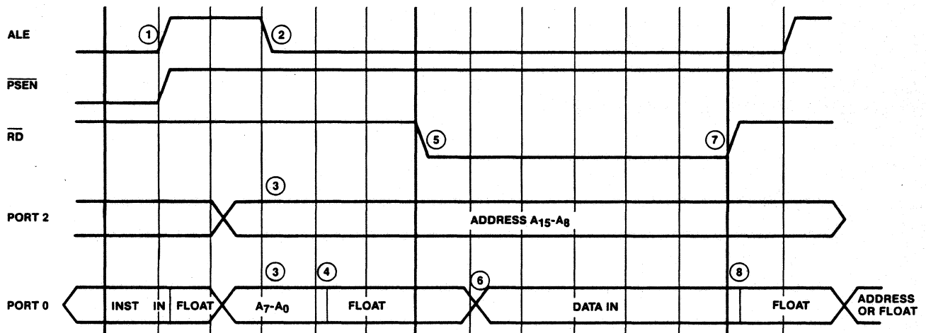
Figure 2.42. Data Memory Read Cycle Timing
