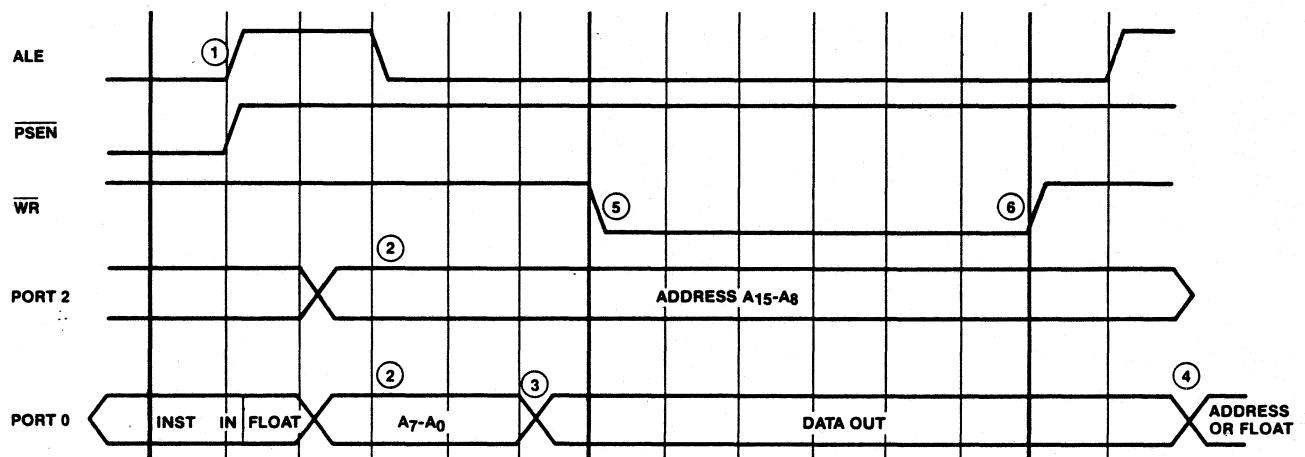
Figure 2.43. Data Memory Write Cycle Timing
