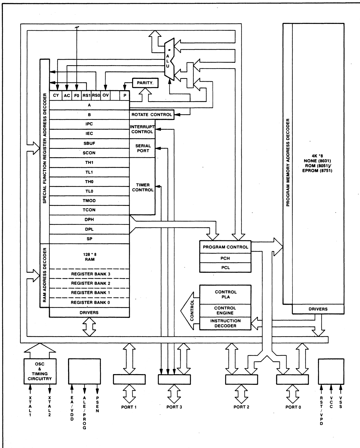
Figure 2.11. 8051 Family Functional Block Diagram
