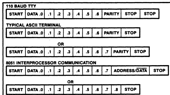
Figure 2.52. Typical Frame Formats
