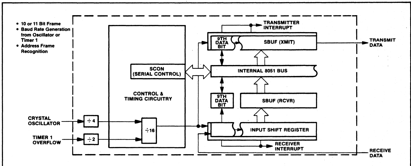
Figure 2.6. Serial Port—UART Modes 1, 2, and 3
