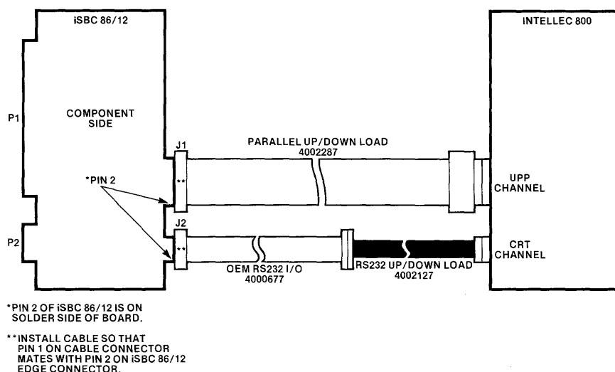
Figure 2-4. iSBC 86/12 to Intellec 800 CRT Channel Cabling
