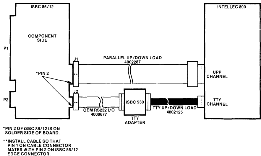
Figure 2-3. iSBC 86/12 to Intellec 800 TTY Channel Cabling
