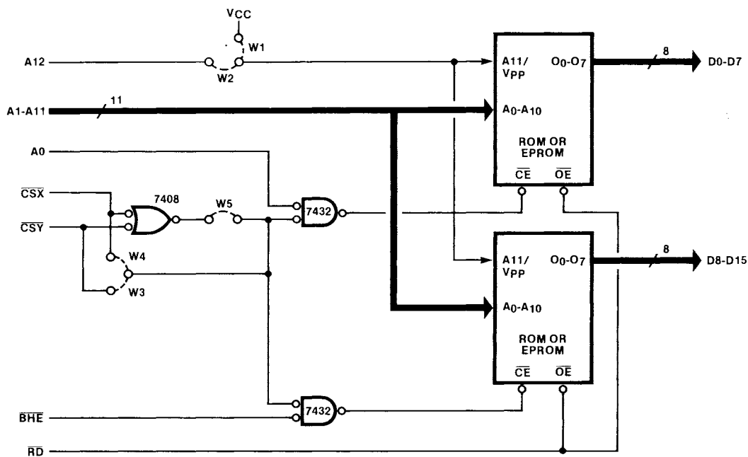
Figure C-3. Design Example 2
