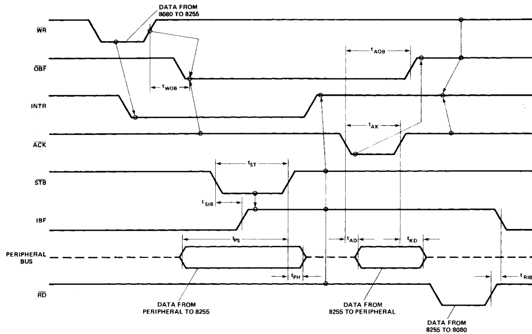
Figure 30. MODE 2 (Bidirectional)
