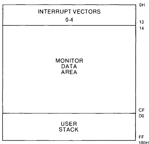
Figure 4-1. Reserved Memory
