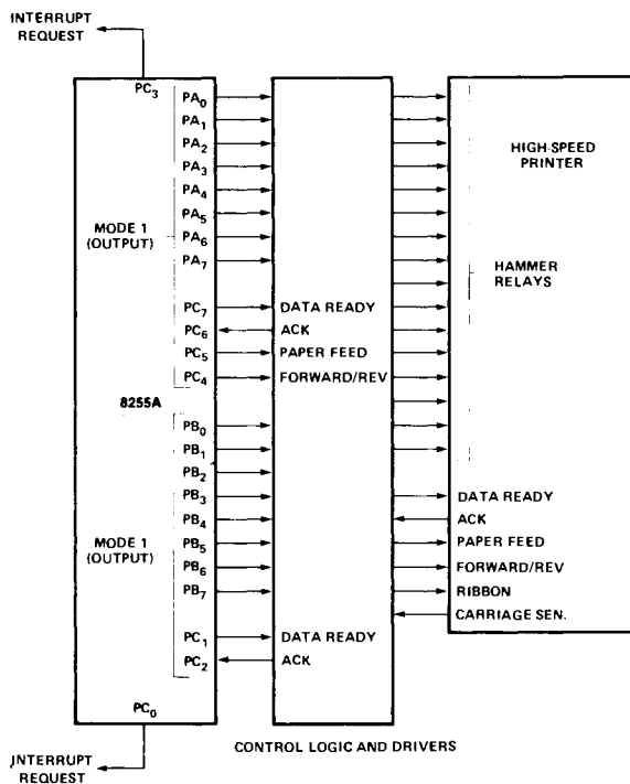
Figure 17. Printer Interface
