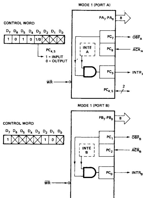
Figure 8. MODE 1 Output
