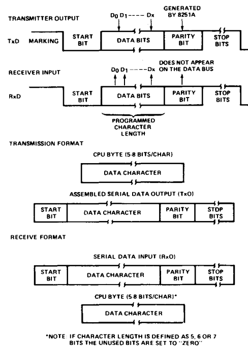
Figure 7. Asynchronous Mode
