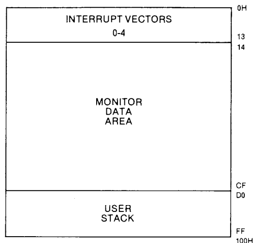
Figure 3-2. Reserved Memory
