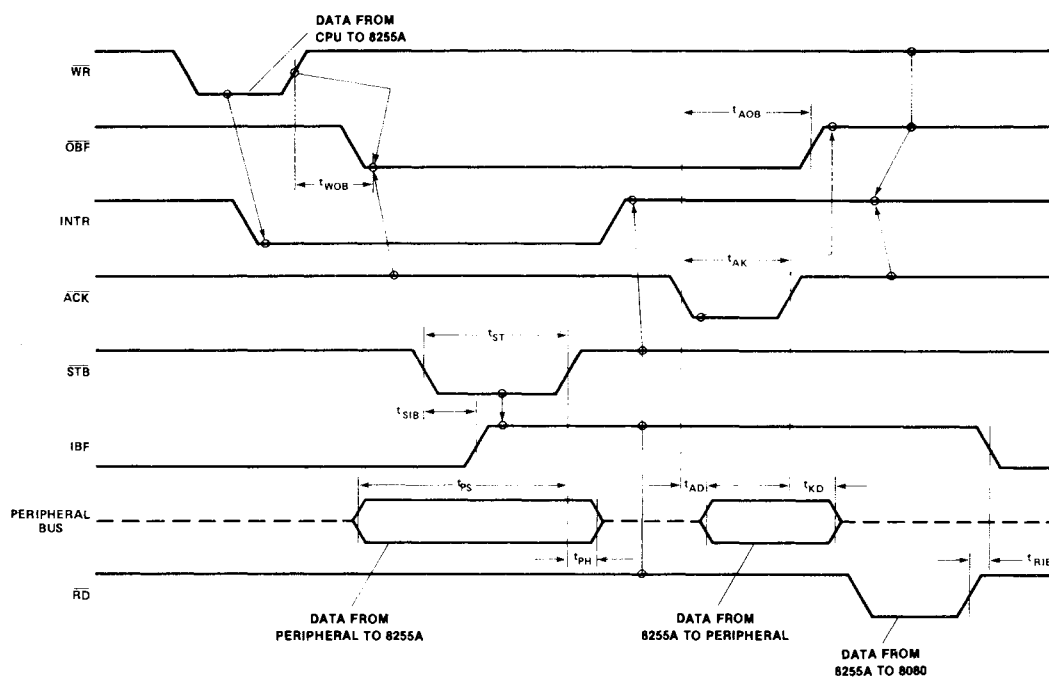
Figure 13. MODE 2 (Bidirectional)
