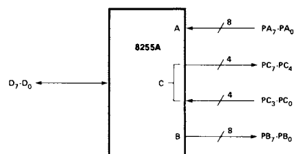
CONTROL WORD #10
