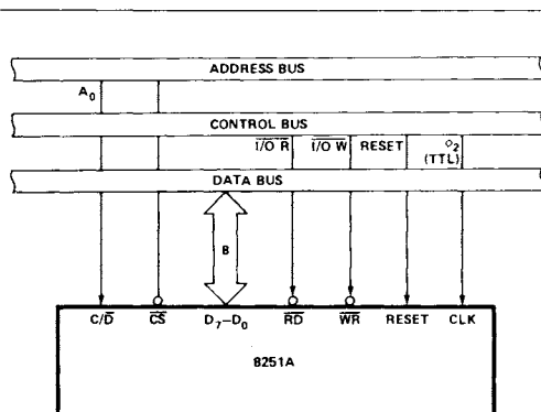
Figure 4. 8251A Interface to 8080 Standard System Bus
