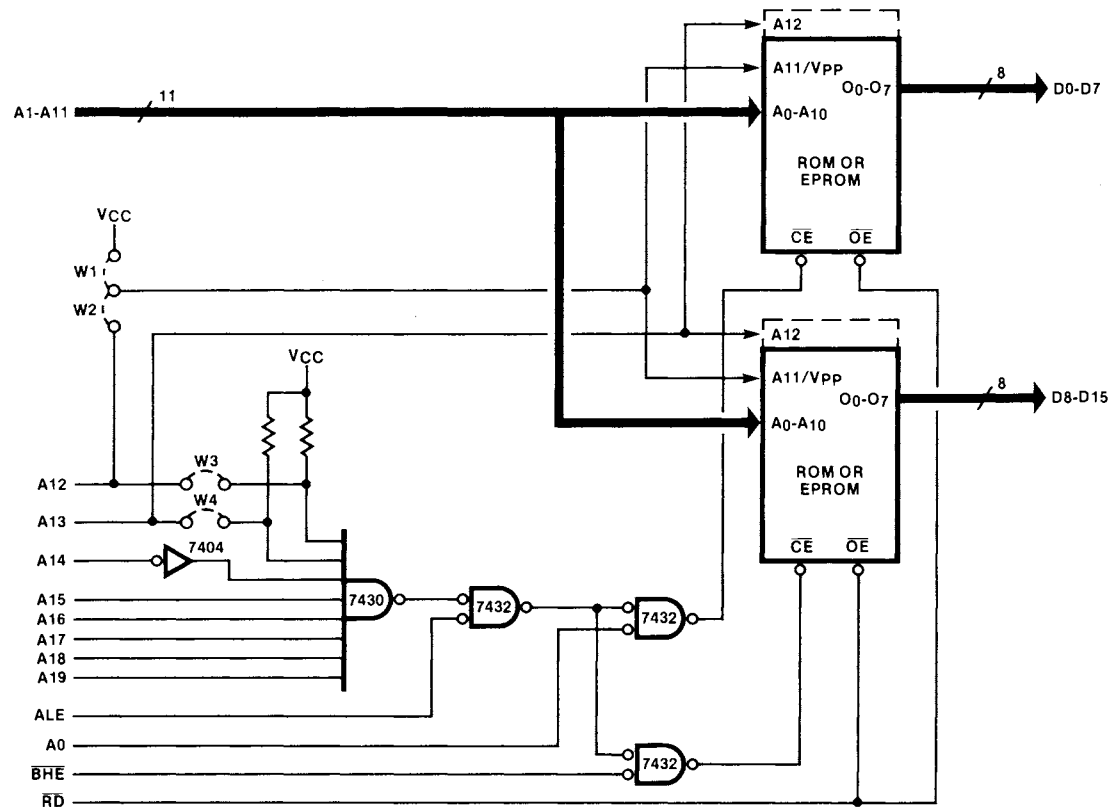
Figure C-2. Design Example 1
