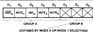
Figure 16. MODE 2 Status Word Format
