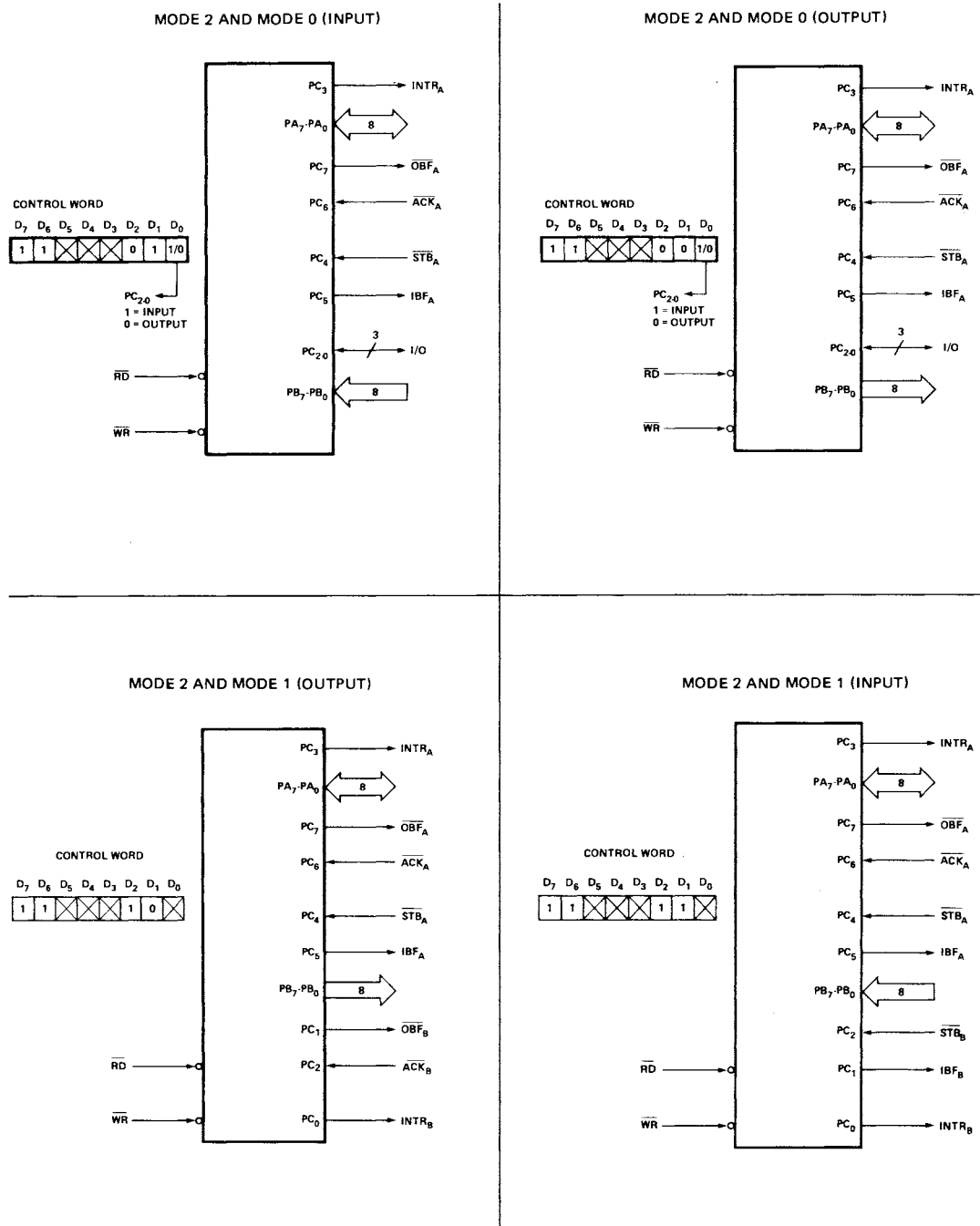
Figure 14. MODE 2 Combinations
