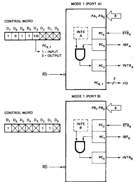
Figure 6. MODE 1 Input
