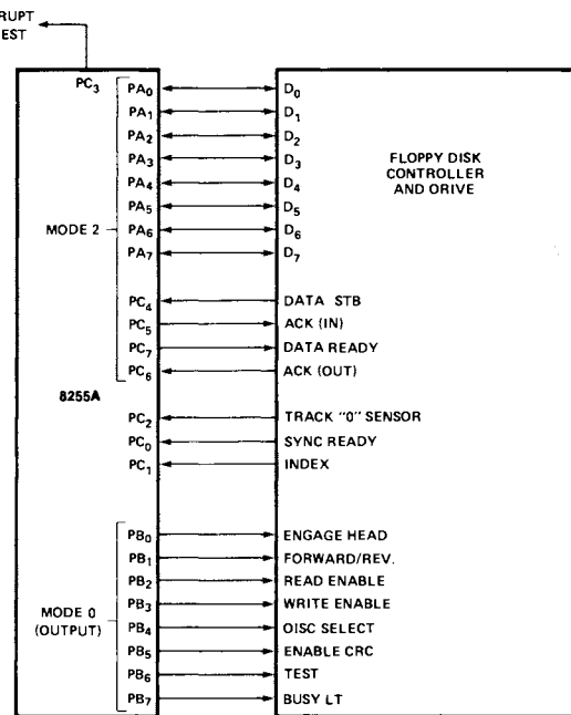
Figure 22. Basic Floppy Disc Interface
