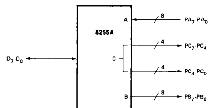
CONTROL WORD #9
