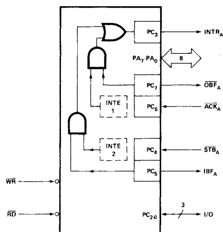
Figure 12. MODE 2
