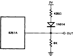
Figure 16. Test Load Circuit
