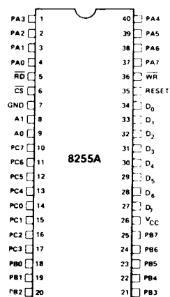
PIN CONFIGURATION
