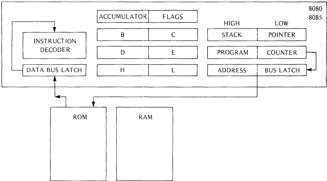
Figure 1-4. Instruction Fetch
