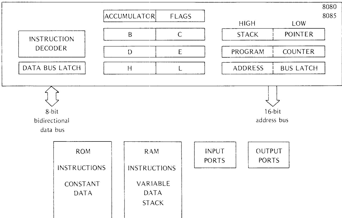
Figure 1-3. 8080/8085 Internal Registers
