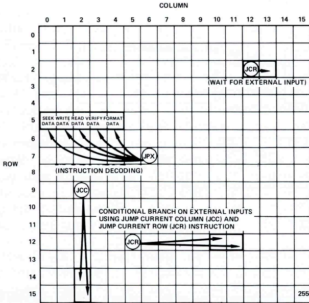
Figure 3. MCU Jump Map for instruction decoding and conditional branching on external inputs
