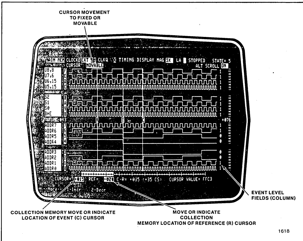
Figure 3. Timing Diagrams
