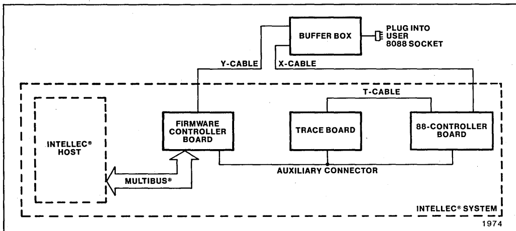
Figure 1. ICETM-88A Emulator Block Diagram
