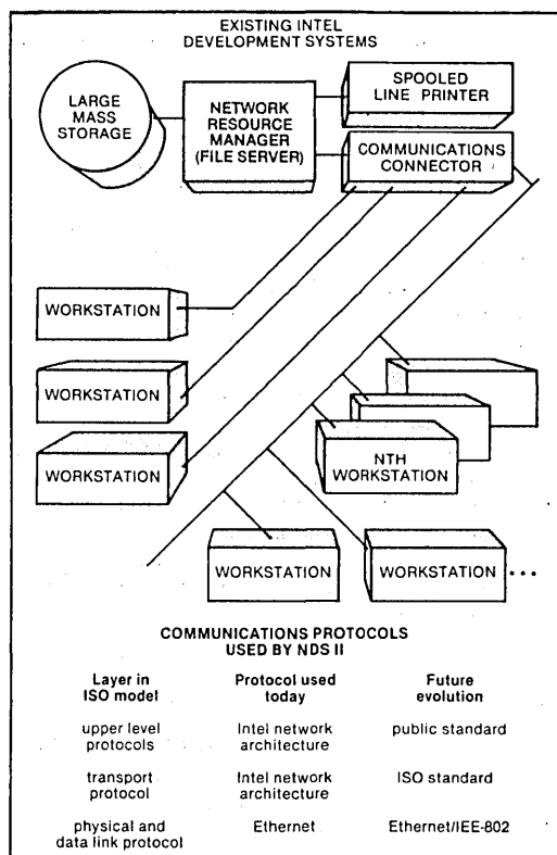
Fig. 4. An LAN can integrate shared and dedicated software-development resources. A shared, central database allows the storage and management of project information. Dedicated, single-user workstations provide team members with processing power, large memory space and quick response. An LAN linking individual workstations furnishes communications between software developers and common access to database information through a network resource manager. An efficient LAN, such as Intel's NDS-II, will eventually be able to connect workstations from different manufacturers to serve changing software-development needs. This goal, however, requires further standardization of communications protocols, the aim of the International Standards Organization (ISO) and other groups.
