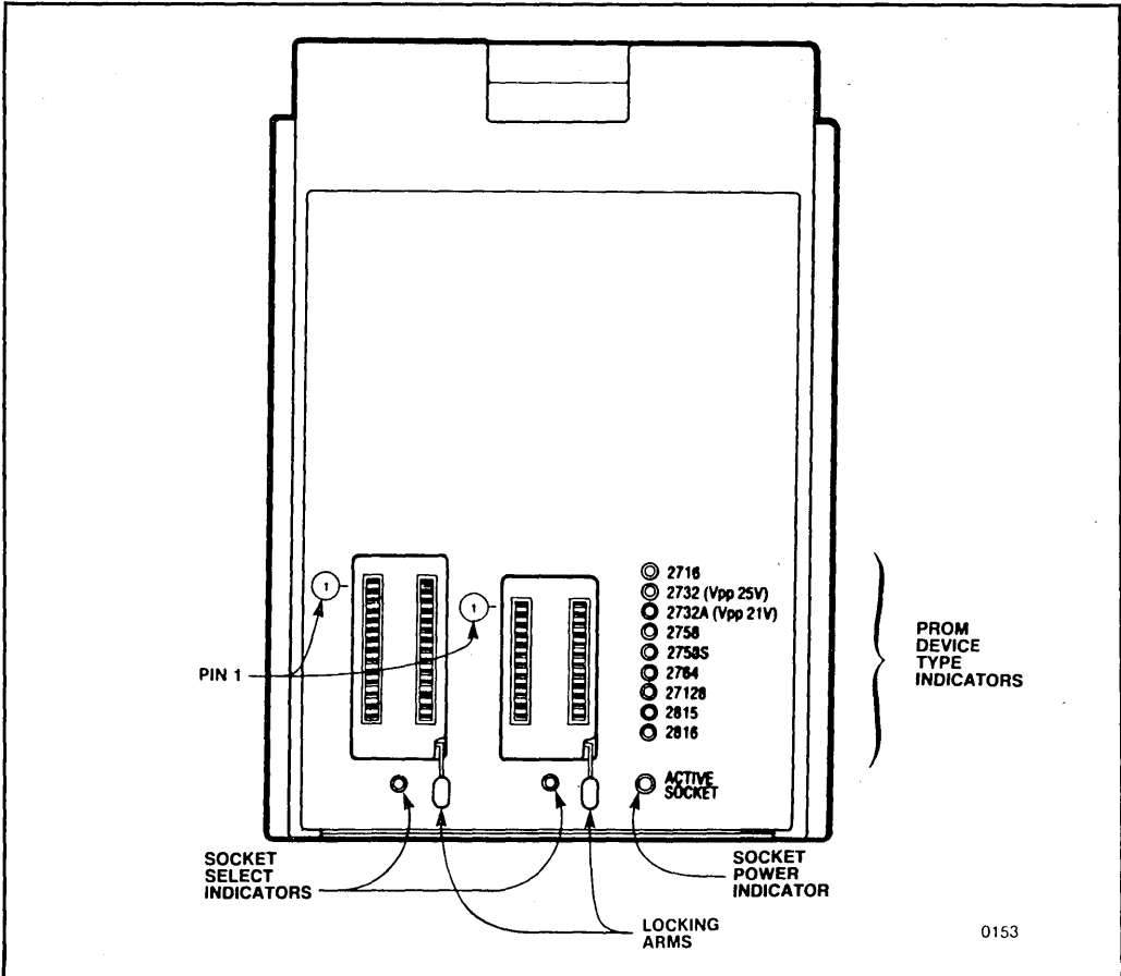
Figure 4. iUP-F27/128 Personality Module
