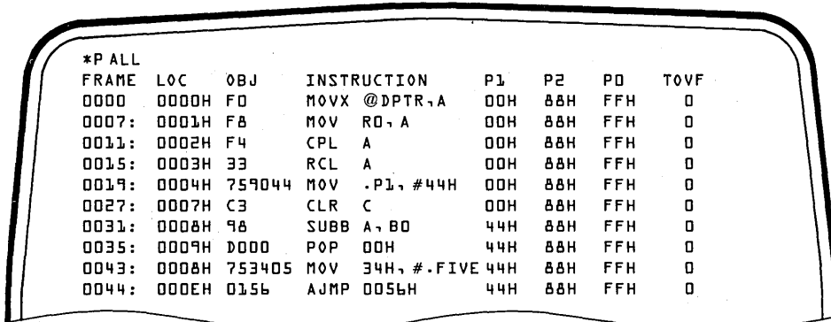
Figure 2. Sample Trace Display in Instruction Mode
