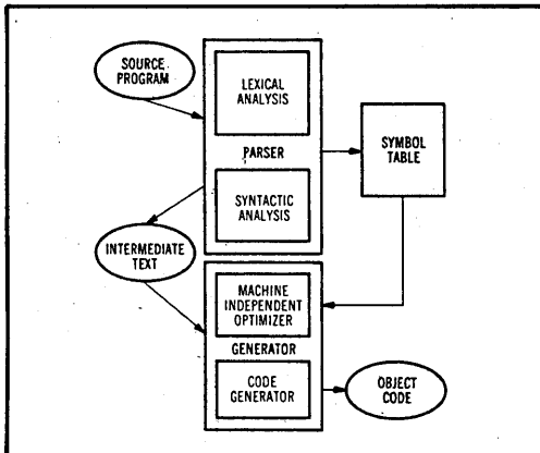
Fig 2 Compilation process. Parsing of source program produces symbol table and intermediate text string. Text string is then optimized, resulting in generation of object code
