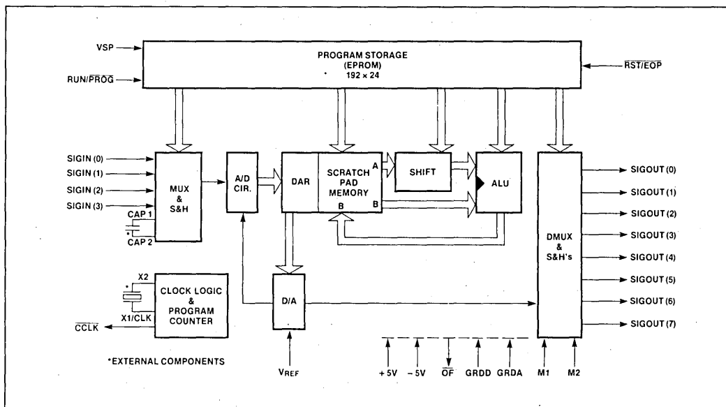
Figure 1. 2920 Function Block Diagram (Run Mode)
