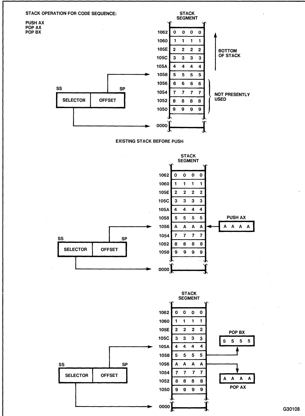
Figure 2-8. Stack Operation
