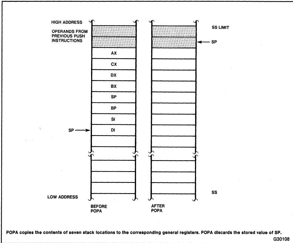
Figure 3-4. POPA
