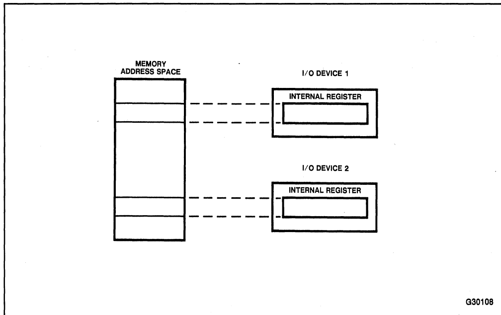
Figure 2-14. Memory-Mapped I/O
