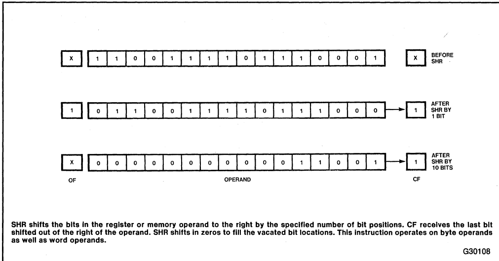
Figure 3-7. SHR
