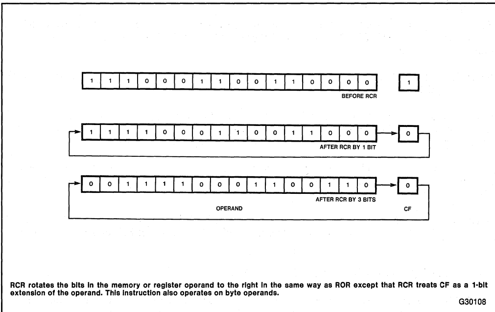
Figure 3-12. RCR
