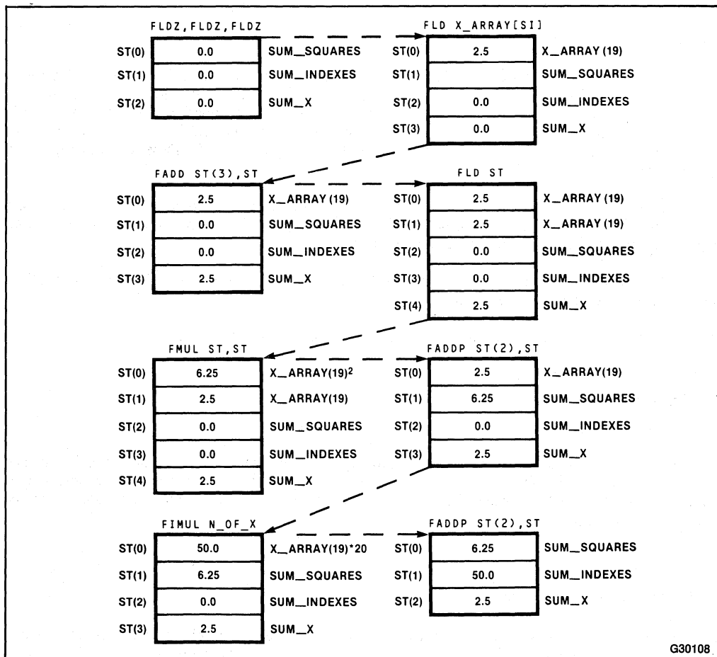
Figure 2-8. Instructions and Register Stack
