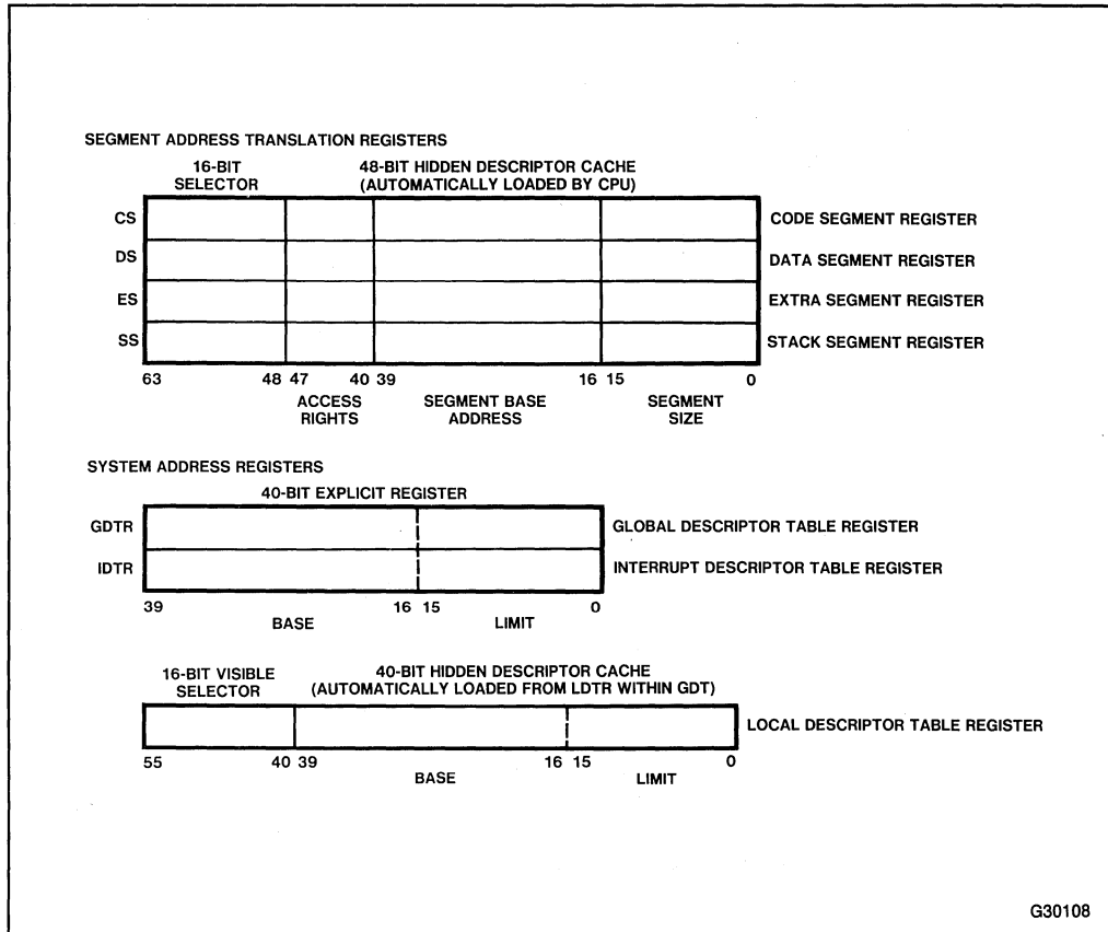
Figure 6-8. Memory Management Registers
