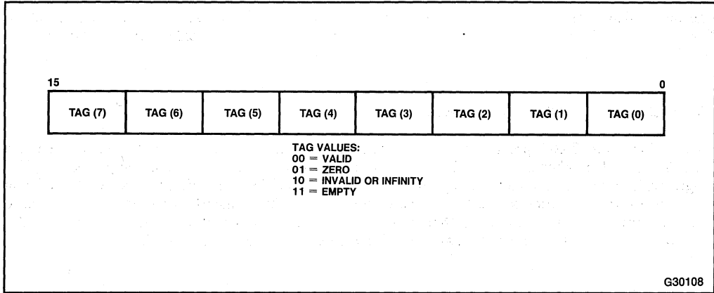
Figure 1-6. 80287 Tag Word Format
