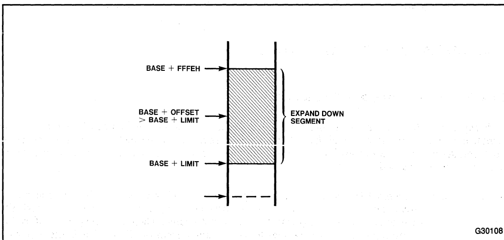
Figure 11-1. Expand-Down Segment
