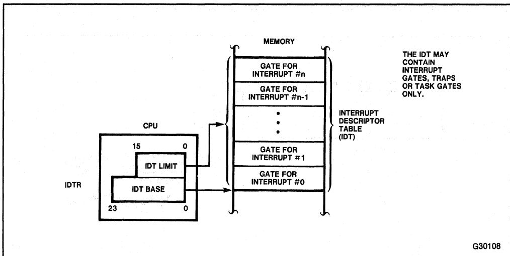
Figure 9-1. Interrupt Descriptor Table Definition
