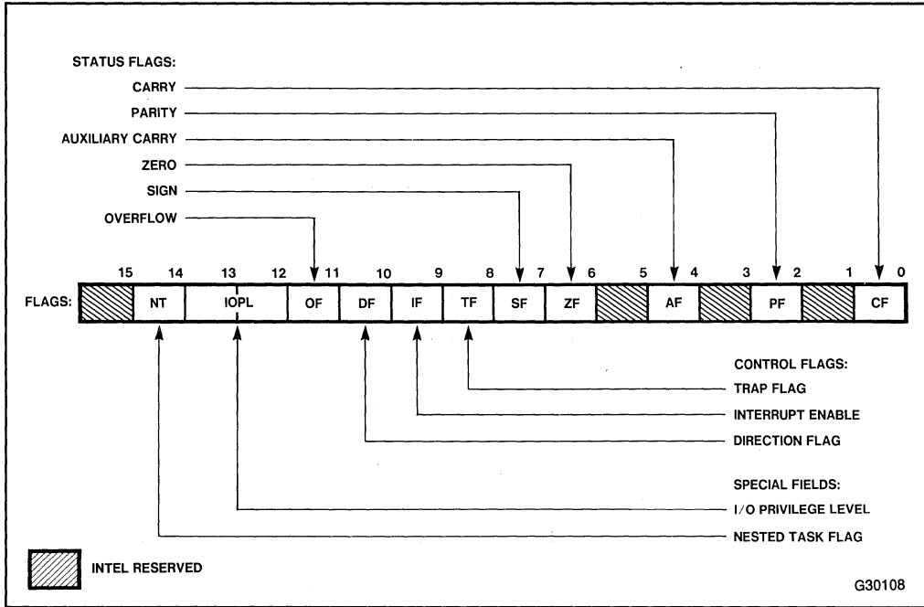
Figure 3-5. Flag Word Contents
