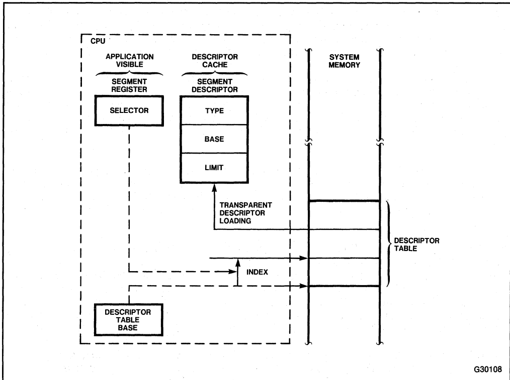
Figure 6-9. Descriptor Loading
