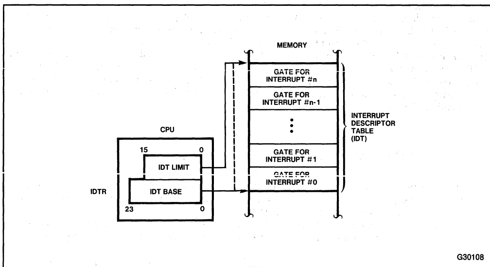
Figure 10-2. Interrupt Descriptor Table Definition
