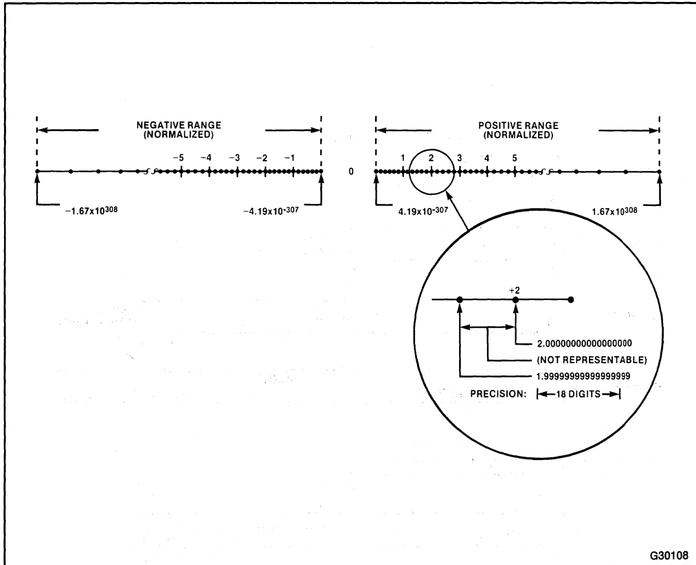
Figure 1-8. 80287 Number System
