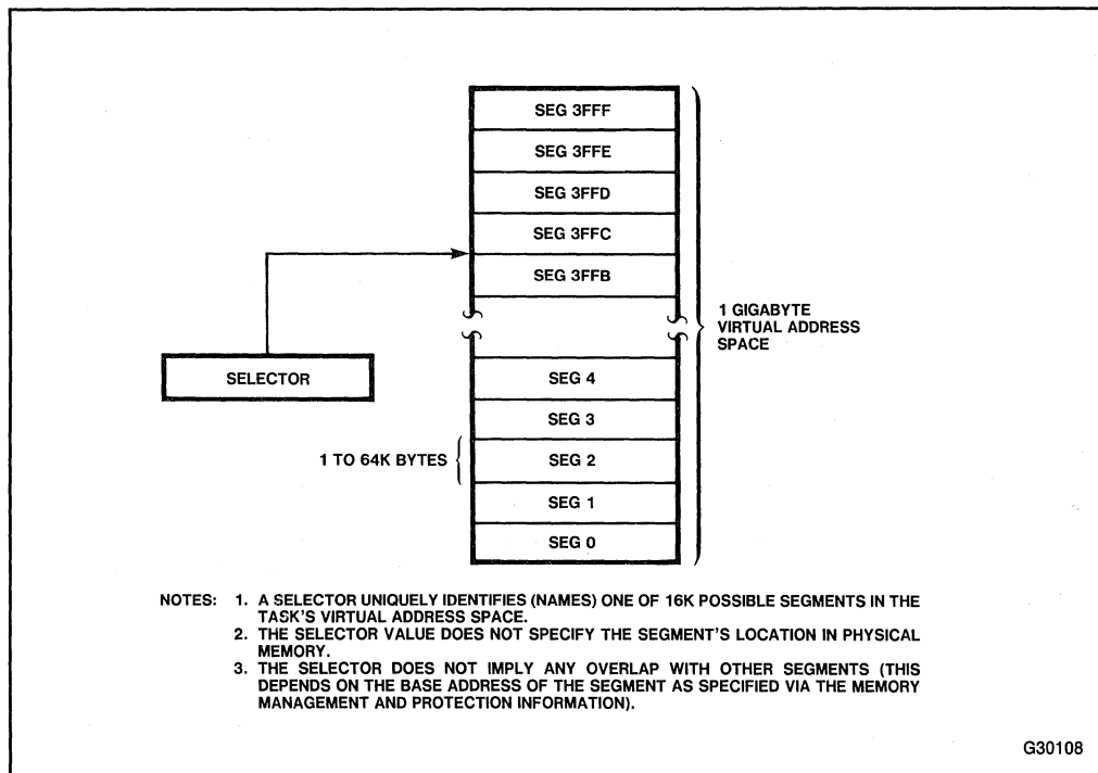
Figure 2-6. Protected Mode Segment Selector Interpretation
