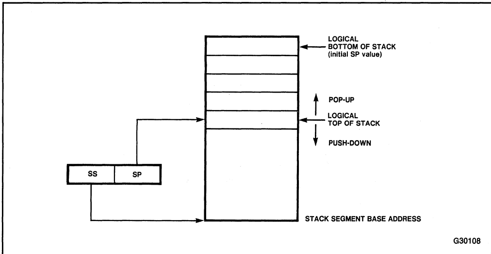
Figure 2-7. 80286 Stack
