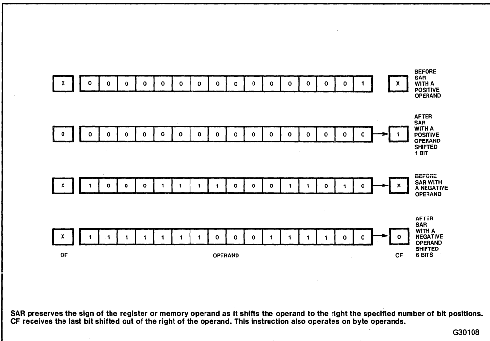
Figure 3-8. SAR
