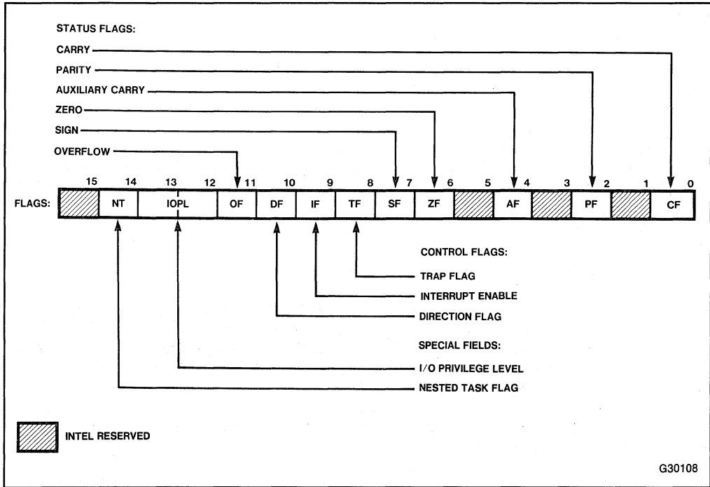
Figure 2-10. Flags Register
