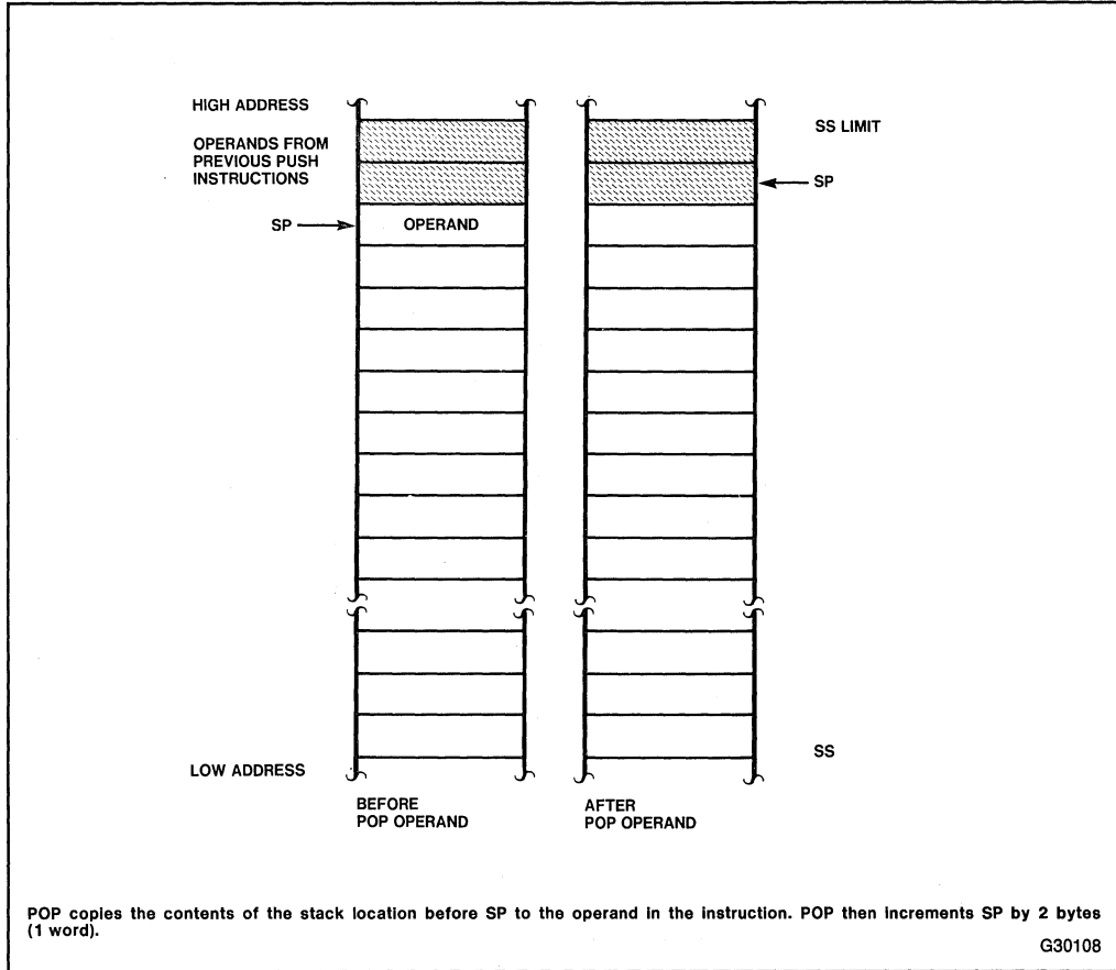
Figure 3-3. POP
