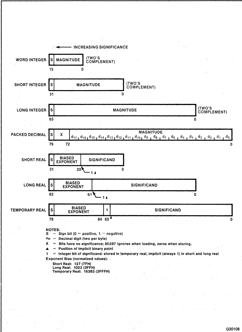
Figure 1-9. Data Formats
