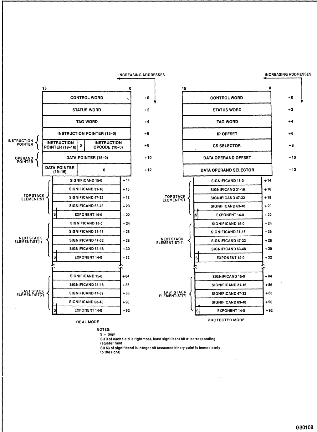
Figure 2-1. FSAVE/FRSTOR Memory Layout
