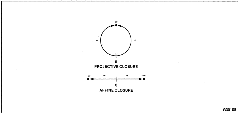
Figure 1-10. Projective versus Affine Closure
