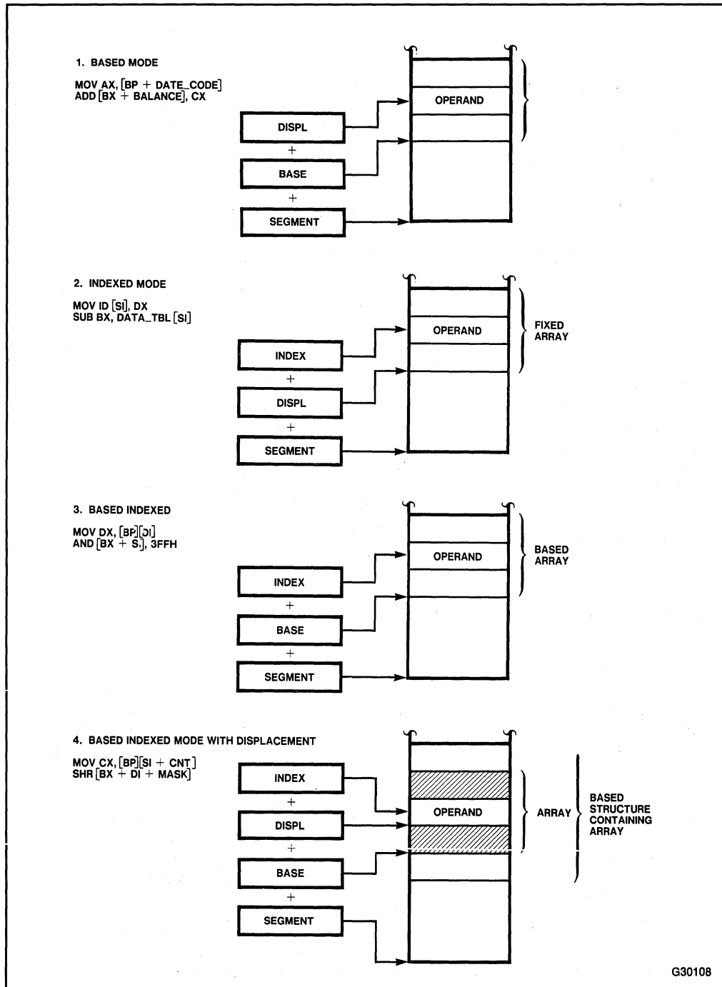
Figure 2-13. Complex Addressing Modes
