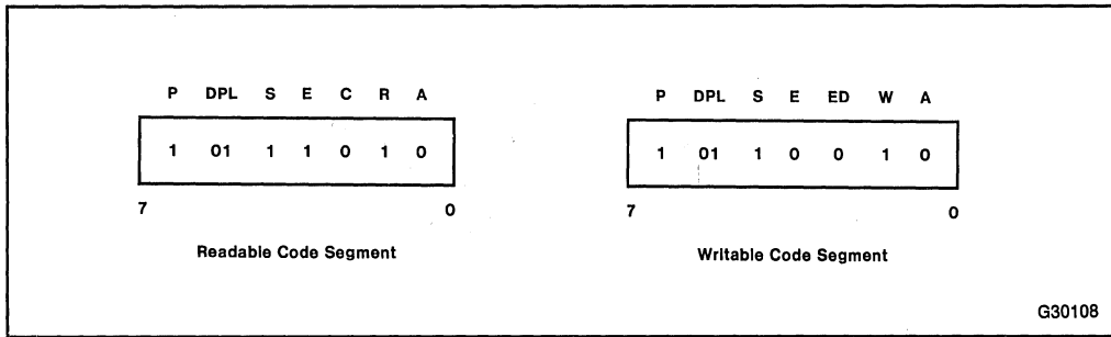
Figure 7-8. Access Byte Examples
