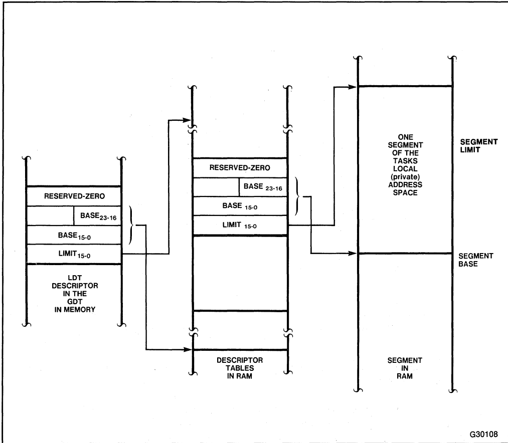
Figure 6-5. LDT Descriptor
