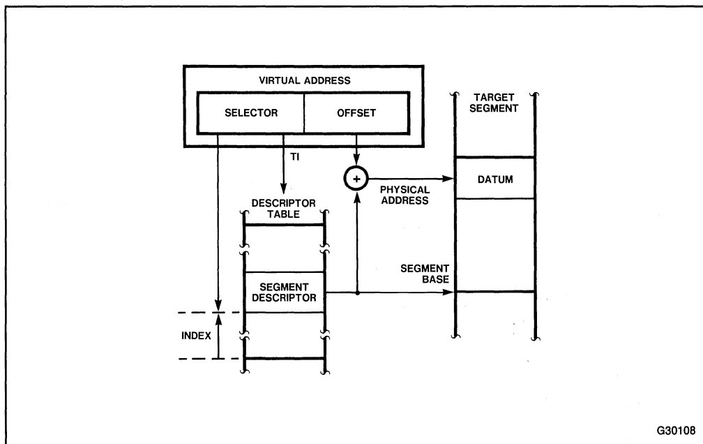
Figure 6-6. Virtual-to-Physical Address Translation
