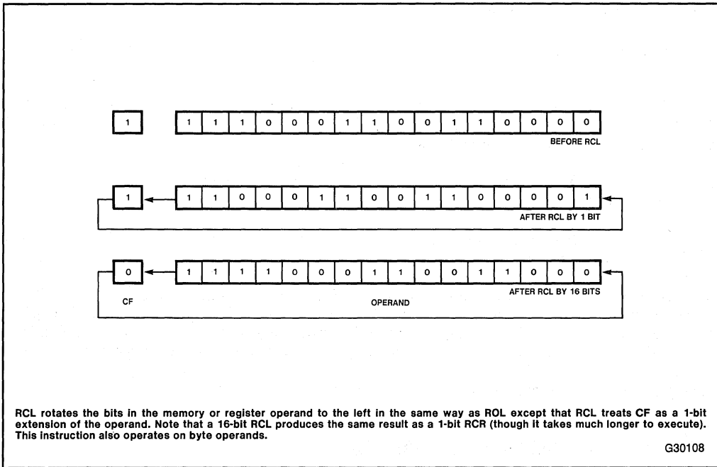
Figure 3-11. RCL
