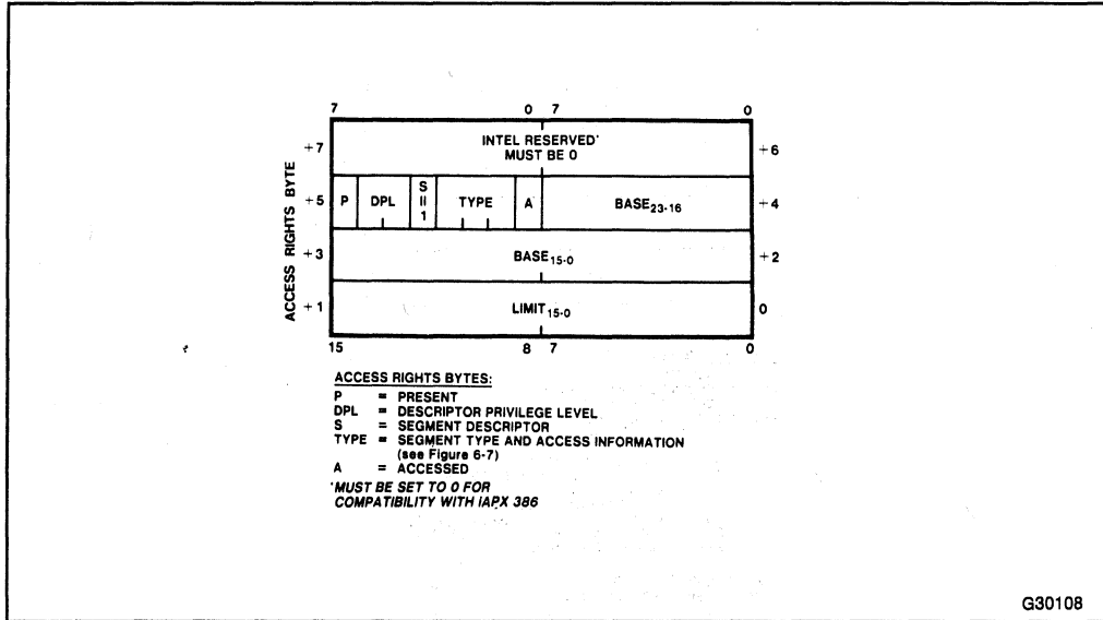
Figure 6-3. Code or Data Segment Descriptor (S = 1)
