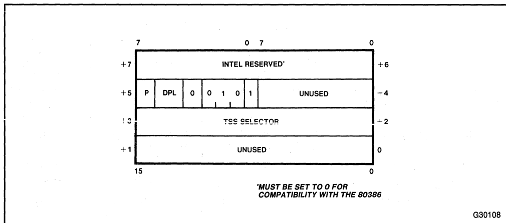
Figure 8-3. Task Gate Descriptor
