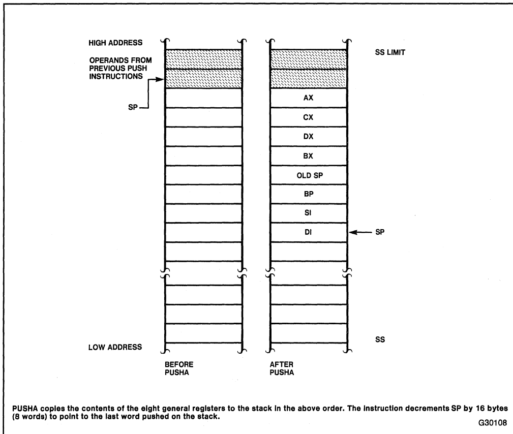
Figure 3-2. PUSH A
