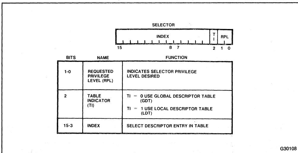
Figure 7-7. Selector Fields
