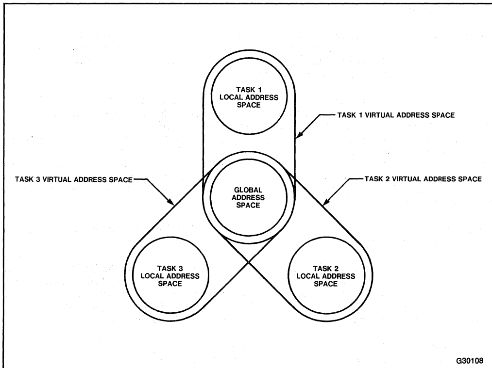
Figure 6-2. Address Spaces and Task Isolation
