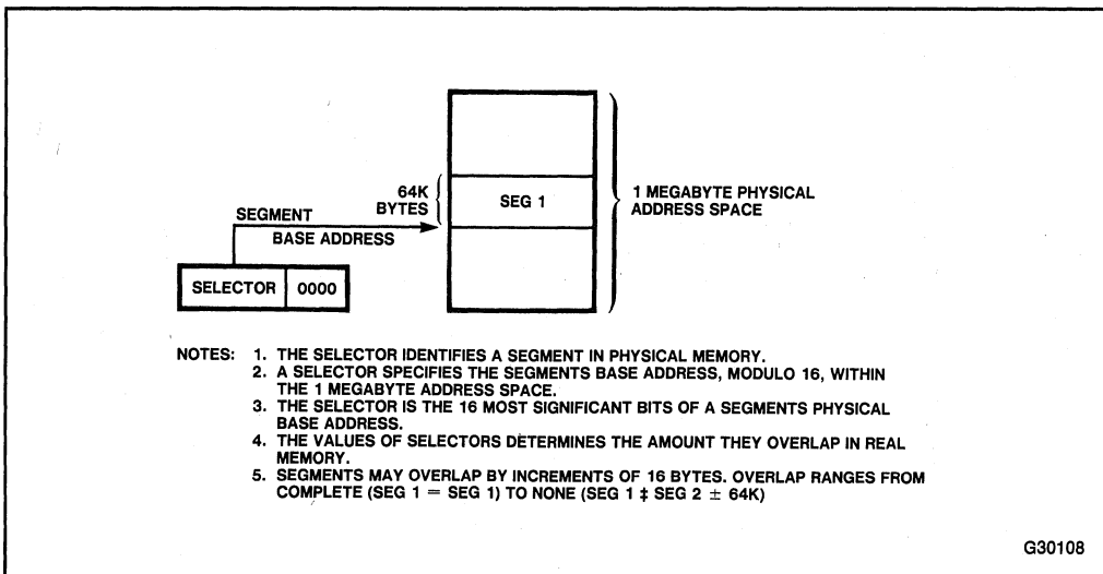
Figure 2-5. Real Address Mode Segment Selector Interpretation
