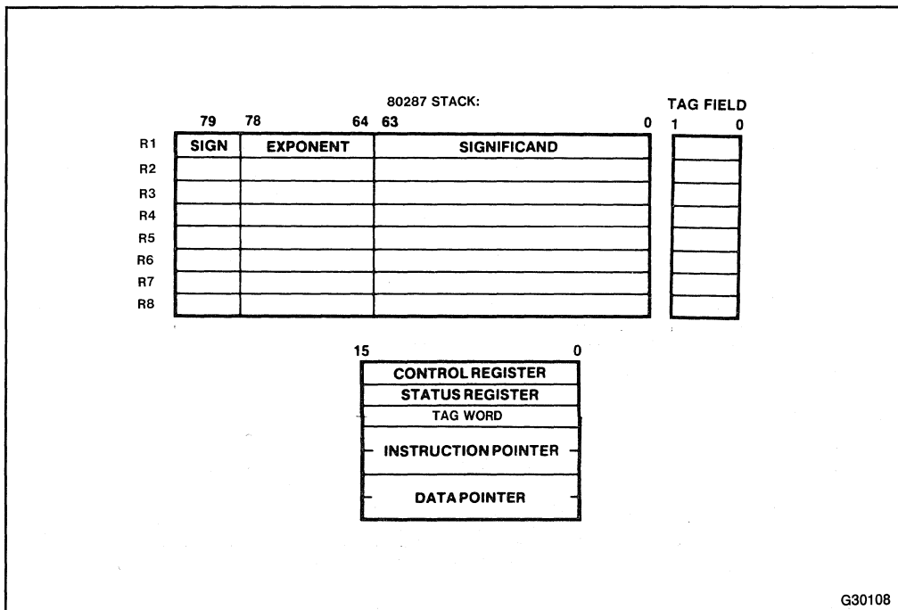
Figure 1-3. 80287 Register Set
