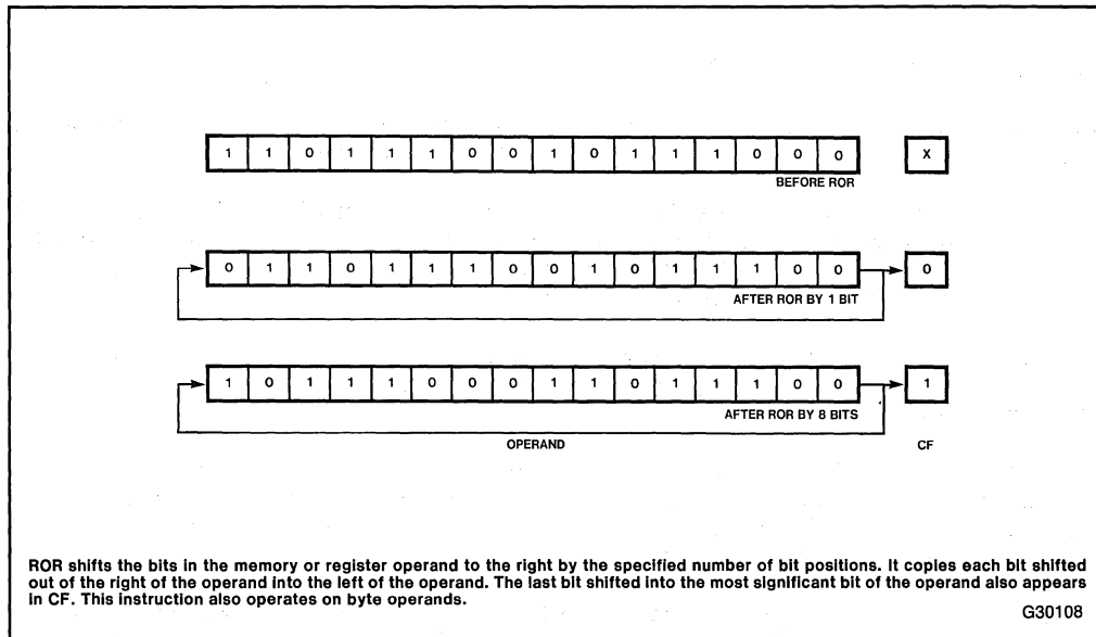
Figure 3-10. ROR
