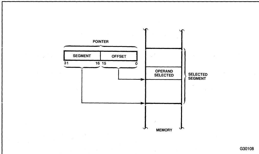
Figure 2-11. Two-Component Address
