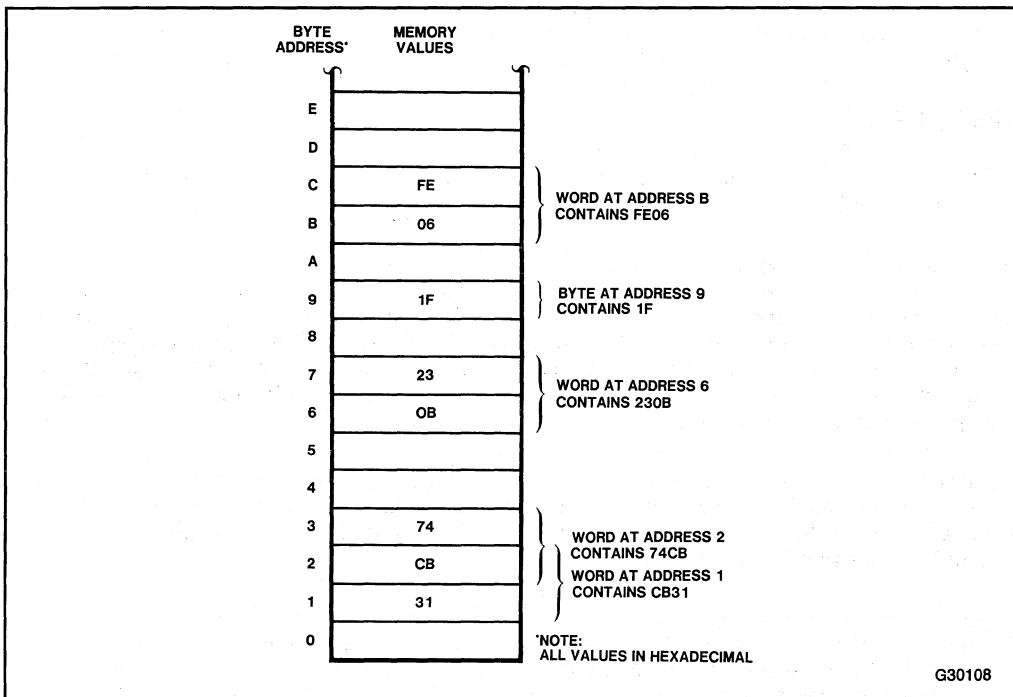
Figure 2-2. Bytes and Words in Memory
