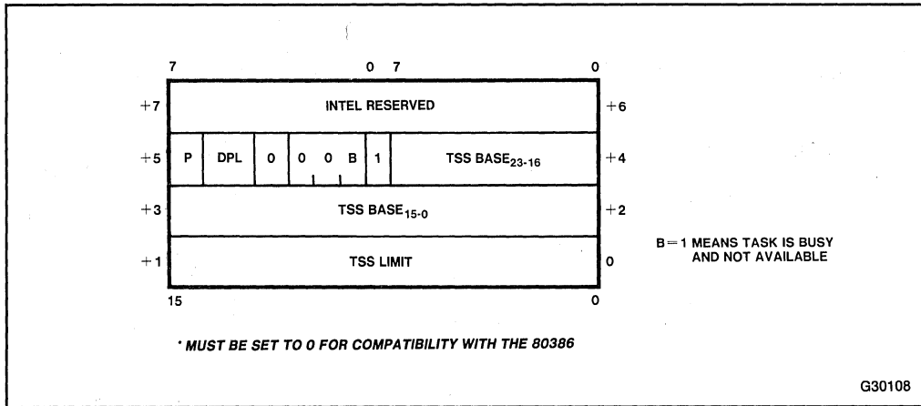
Figure 8-2. TSS Descriptor
