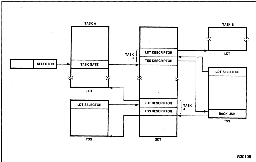
Figure 8-4. Task Switch Through a Task Gate
