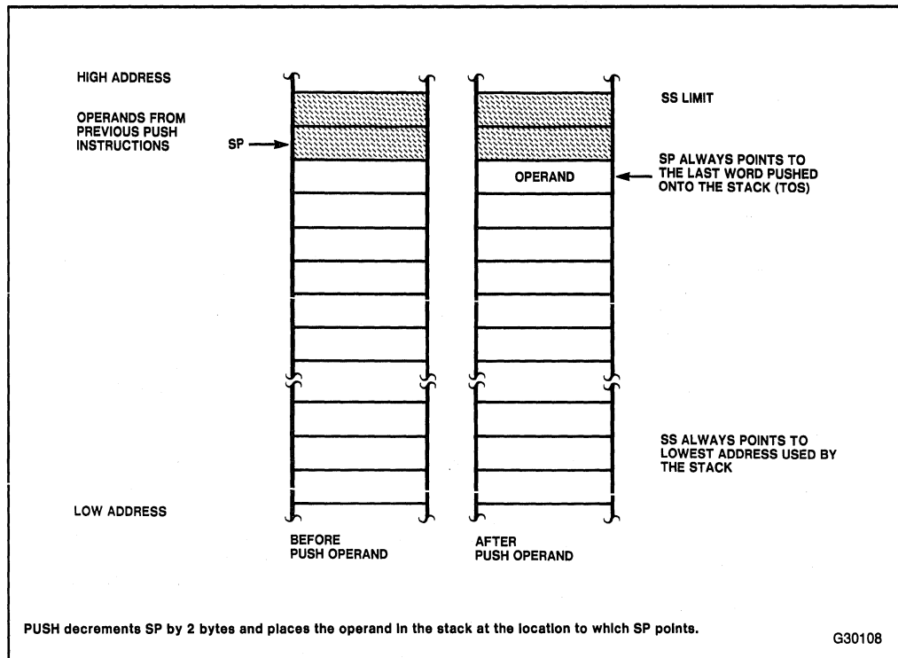
Figure 3-1. PUSH
