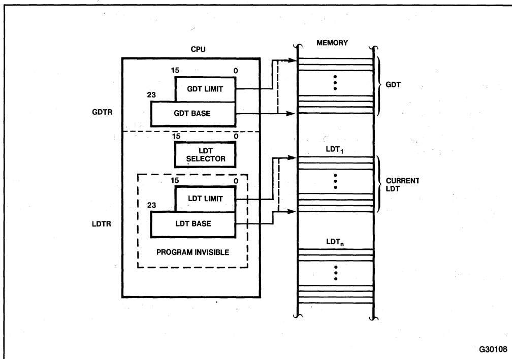
Figure 10-1. Local and Global Descriptor Table Definition
