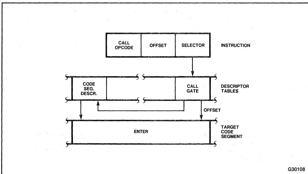
Figure 7-11. Call Gate
