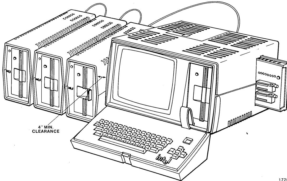
Figure 1-4 System with Options
