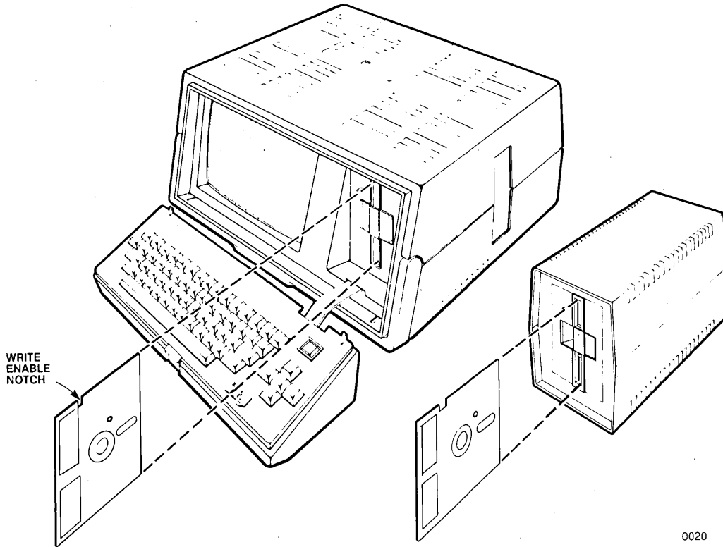
Figure 3-10 Disk Insertion
