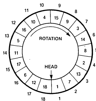
Figure 8-15 Sector Interleaving
