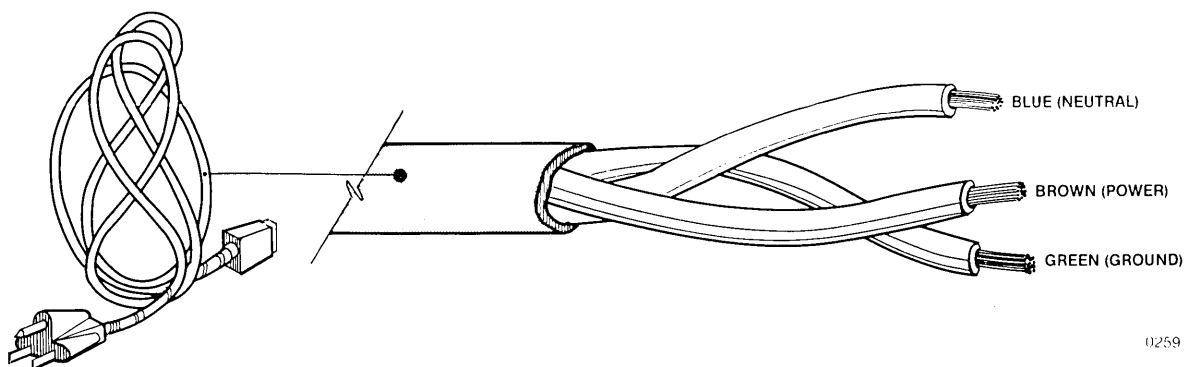
Figure A-3 Power Cable
