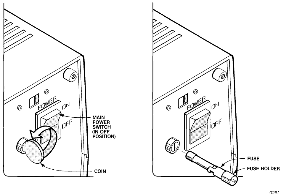
Figure A-6 Changing the Fuse
