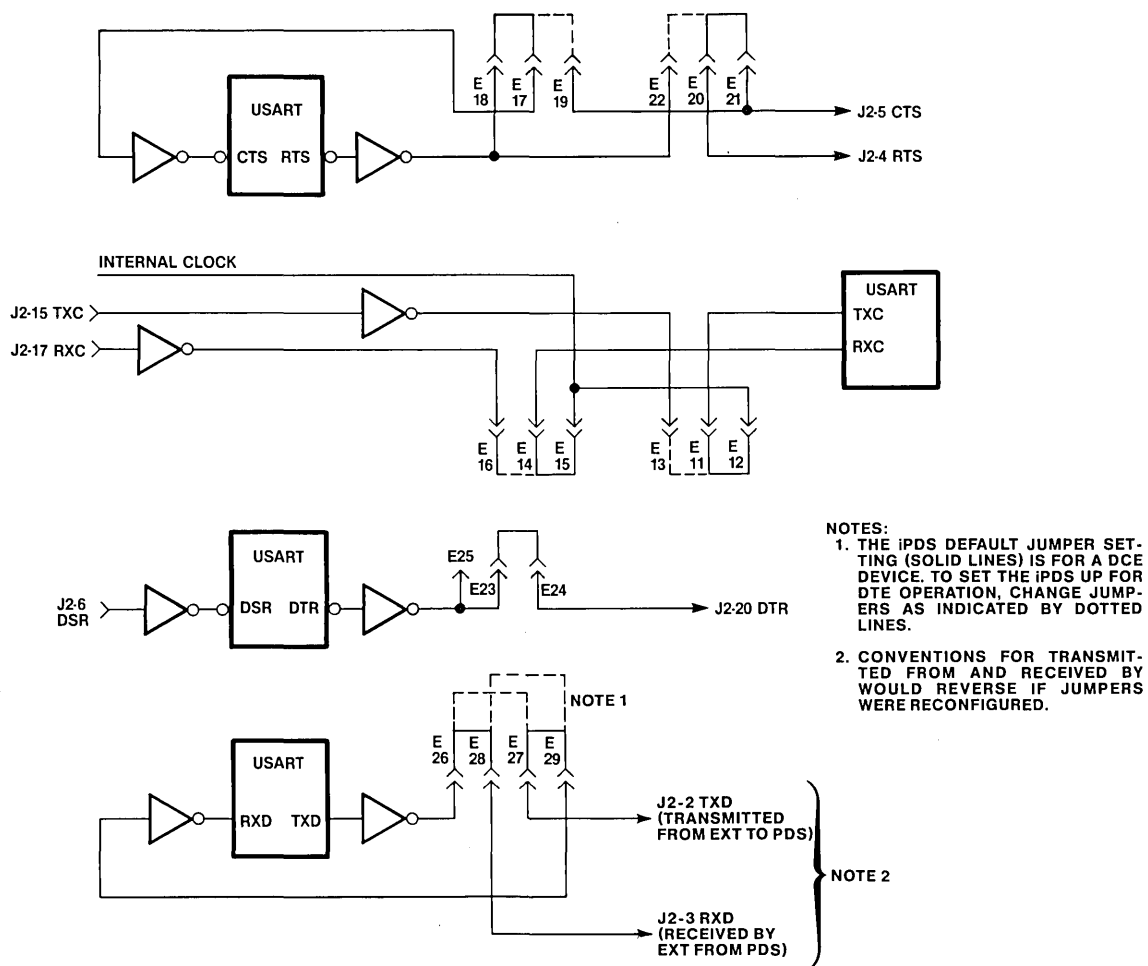
Figure A-10 Schematics for the Serial I/O Interface
