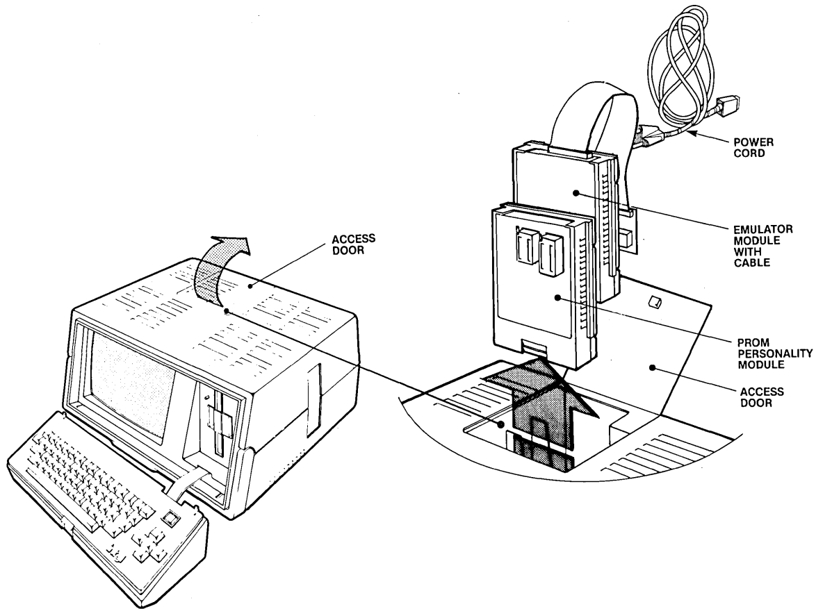
Figure 3-4 Accessing the Storage Area
