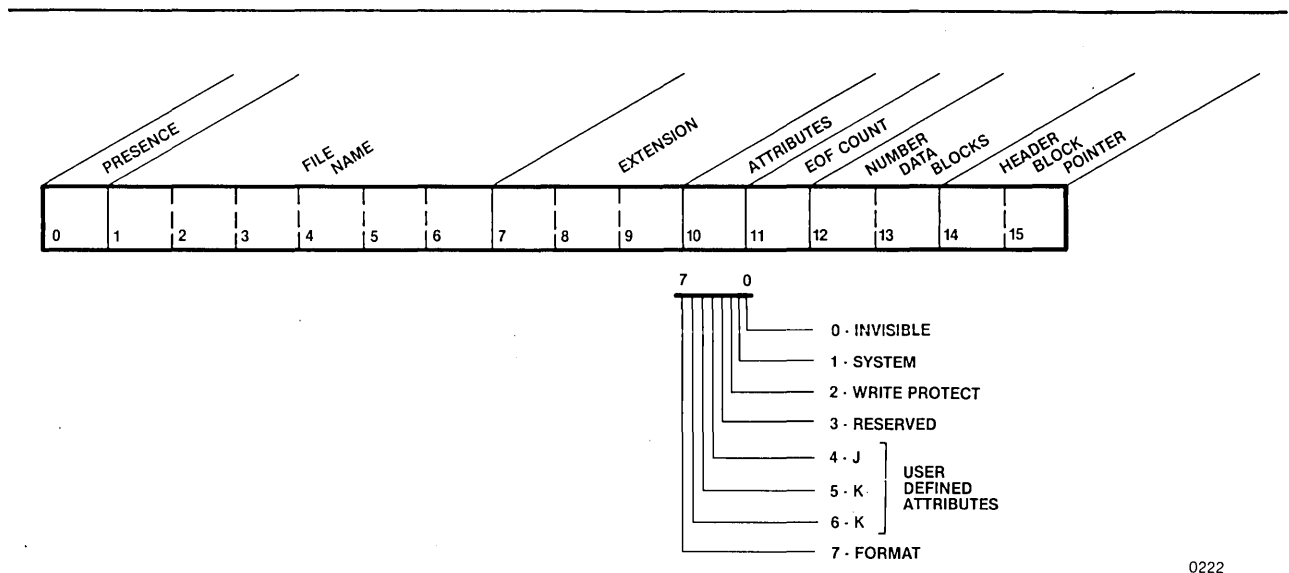
Figure 8-16 Directory Entry
