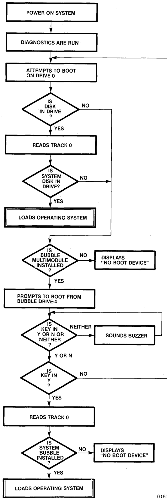
Figure 3-13 Flowchart of Initialization Program
