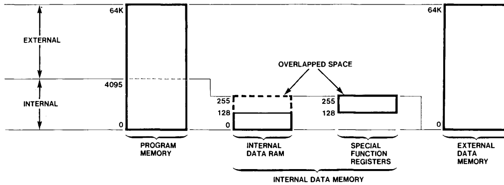
Figure 3-1. 8051 Memory Organization
