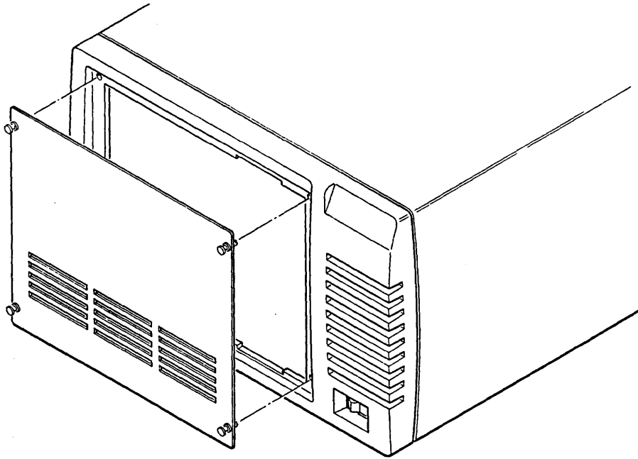
Figure C-1. Front Panel
