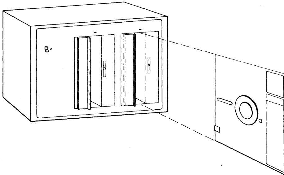
Figure 2-1. Flexible Disk Insertion, Vertical Position
