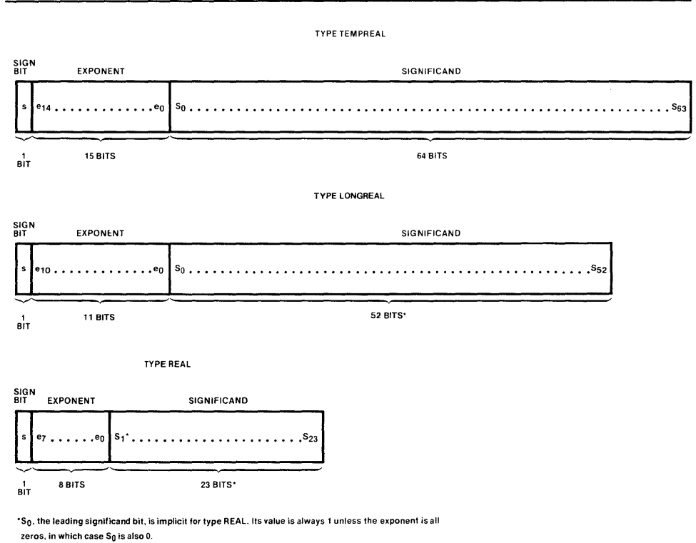
Figure 7-1. Pascal-86 Real Data Types
